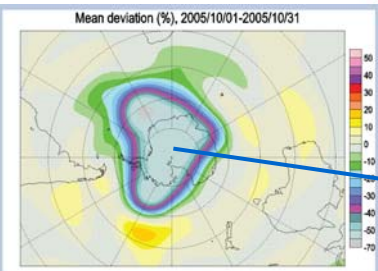
OZONE HOLE & UV
